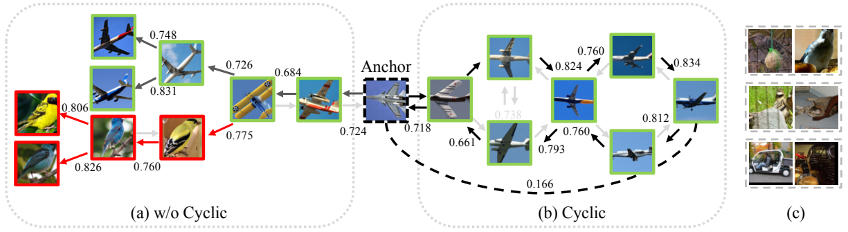
Figure 5: Case study on STL10. (a) vs. (b): Cyclic constraint helps detect erroneous affinity diffusion. (c) Extremely hard positive pairs undiscovered by PAD. Red solid box : with a different class as the anchor; Green solid box : with the same class as the anchor. The numbers above arrows are the corresponding pairwise affinity scores.
